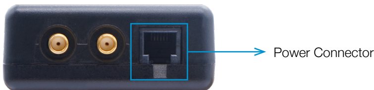
Figure 12: RJ12 power connector on SENTRY
