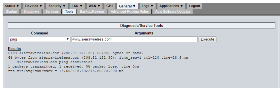
Figure 5-7: Tool example—ping
