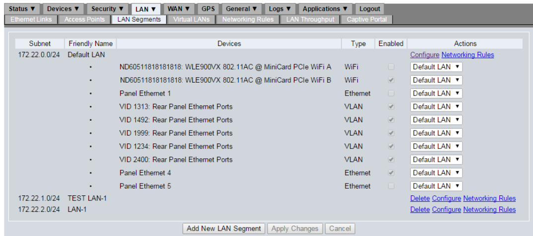
Figure 7-2: Configuring or adding a LAN segment
