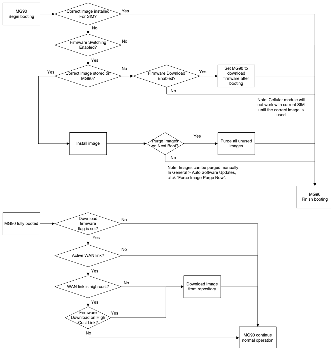
Figure 12-2: Firmware Switching Process
