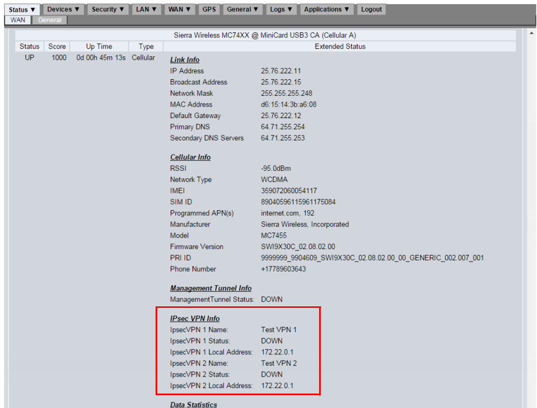
Figure 9-4: Viewing the VPNs assigned to a WAN Link
