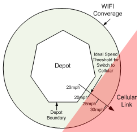
Figure 6-13: Setting a Speed Threshold to Switch to Cellular before Wi-Fi Coverage is lost
