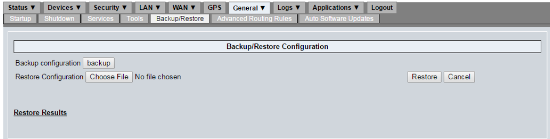
Figure 19-5: LCI: General > Backup/Restore—Sample screen
