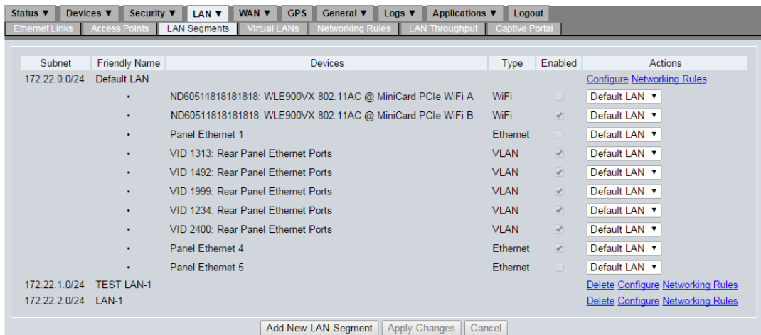
Figure 16-5: LCI: LAN > LAN Segments—Sample screen
