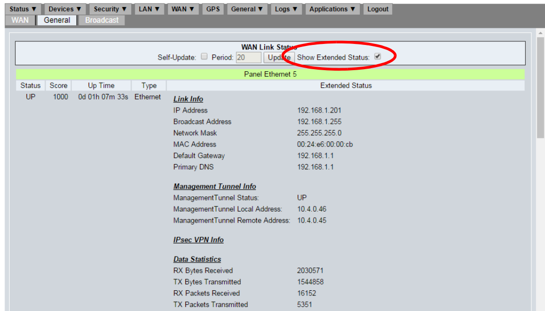
Figure 5-2: LCI: Status > WAN > Extended Status
