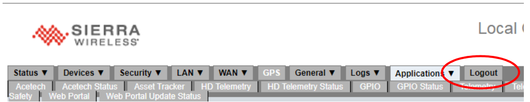
Figure 22-1: Logout Tab
