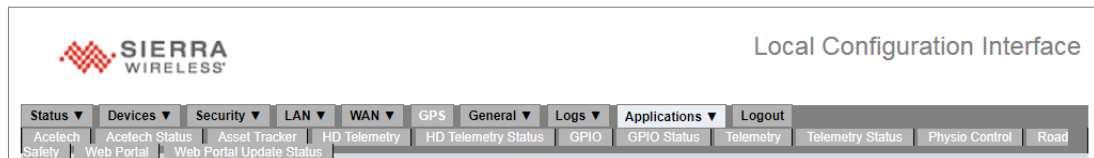
Figure 21-1: Applications Tab
