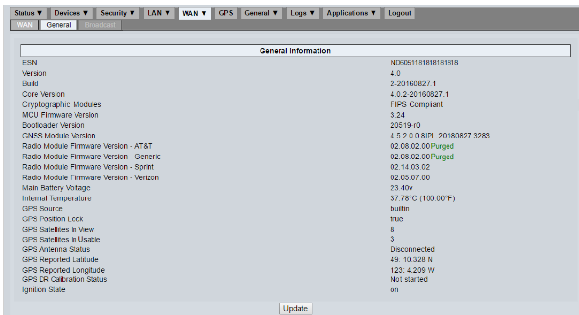
Figure 13-3: General Information screen (Status > General)
