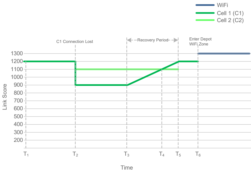
Figure 6-11: Dynamic Priority Timeline—Example
