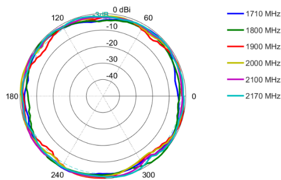
Azimuth: 1710 – 2170 MHz
