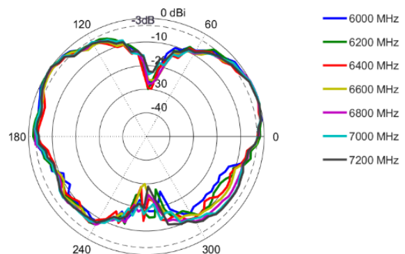
Elevation: 6000 – 7200 MHz
