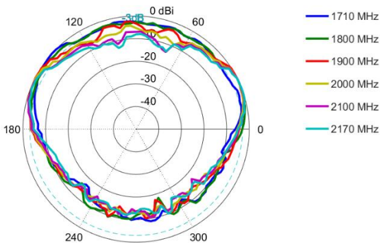
Elevation: 1710 – 2170 MHz
