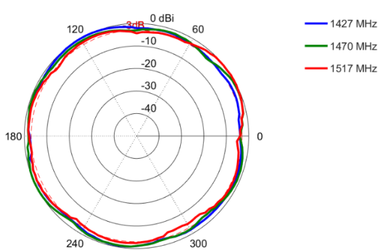
Azimuth: 1427 – 1517 MHz
