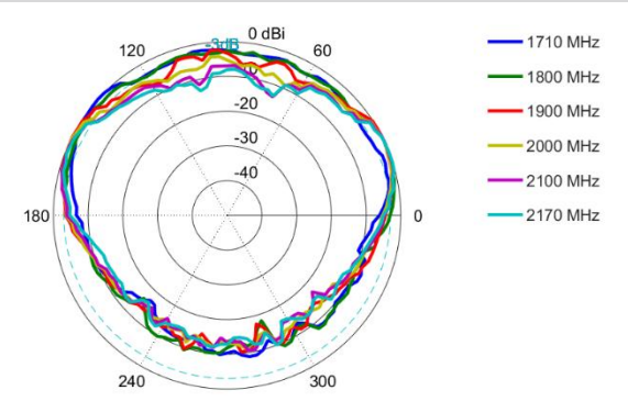
Elevation: 1710 – 2170 MHz
