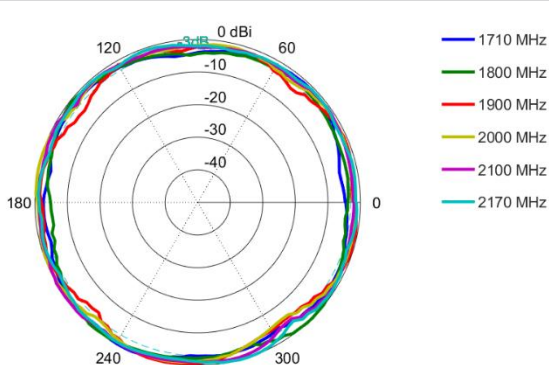
Azimuth: 1710 – 2170 MHz
