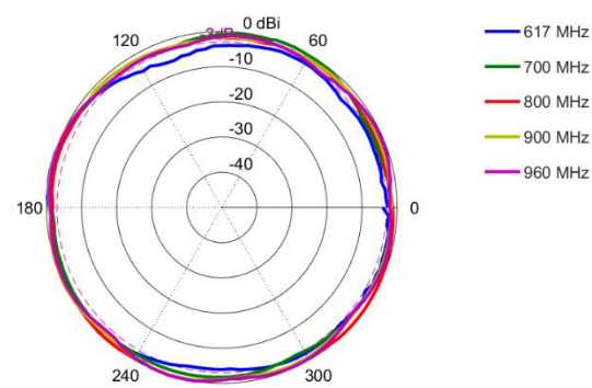
Azimuth: 617 – 960 MHz
