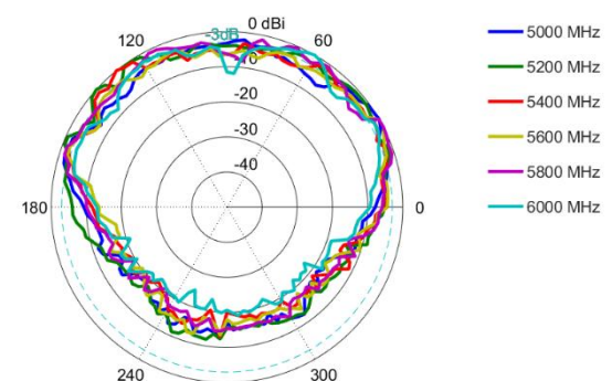
Elevation: 5000 – 6000 MHz
