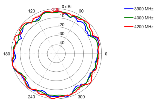
Azimuth: 3900 – 4200 MHz
