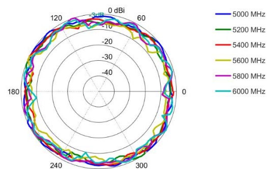
Azimuth: 5000 – 6000 MHz
