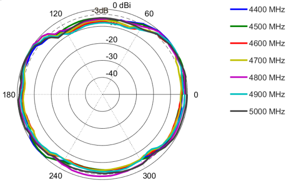
Azimuth: 4400 – 5000 MHz
