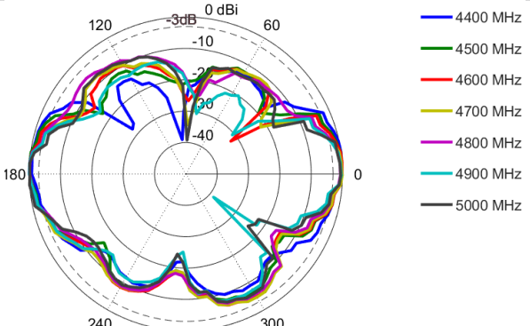
Elevation: 4400 – 5000 MHz
