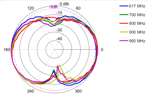
Elevation: 617 – 960 MHz
