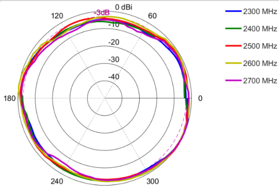
Azimuth: 2300 – 2700 MHz
