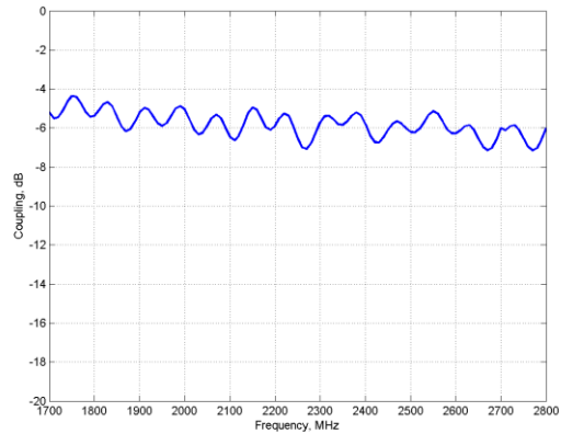
Coupling to internal modem antenna
