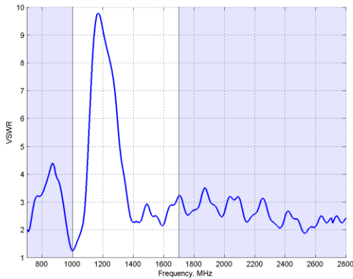
VSWR (coupled)
